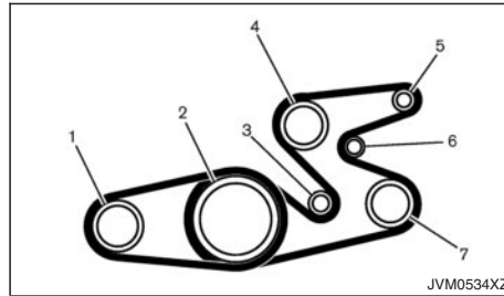
M9T 2.3DCI-Motor
